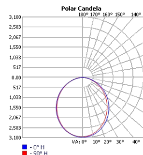
TECHOLED-BX-2-D-8-HI-30
