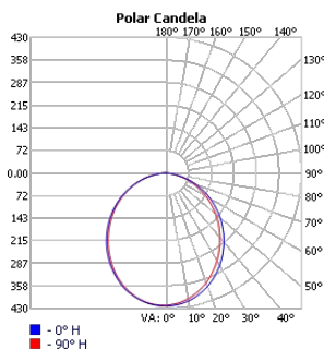
TECHOLED-BX-2-D-2-LO-30
