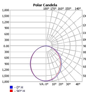
TECHOLED-BX-2-D-8-LO-30
