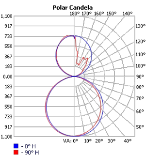
TECHOLED-BX-2-DI-8-LO-30
