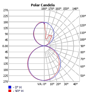
TECHOLED-BX-2-DI-2-LO-30
