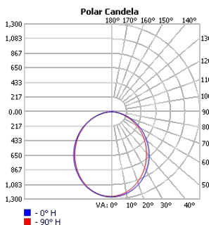
TECHOLED-BX-2-D-6-LO-30
