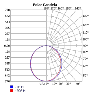
TECHOLED-BX-2-D-2-HI-30
