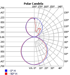
TECHOLED-BX-2-DI-8-ME-30
