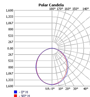
TECHOLED-BX-2-D-4-HI-30
