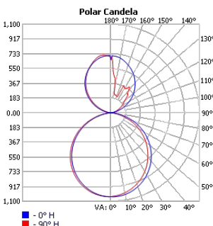
TECHOLED-BX-2-DI-4-HI-30
