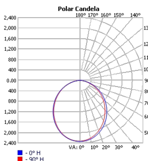
TECHOLED-BX-2-D-8-ME-30
