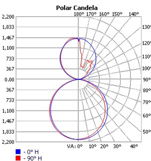
TECHOLED-BX-2-DI-8-HI-30
