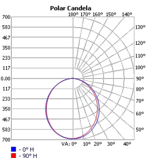
TECHOLED-BX-2-D-2-ME-30
