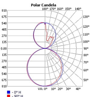
TECHOLED-BX-2-DI-4-ME-30
