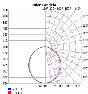
TECHOLED-BX-2-D-4-LO-30
