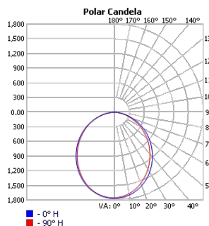
TECHOLED-BX-2-D-6-ME-30
