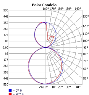
TECHOLED-BX-2-DI-4-LO-30
