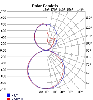
TECHOLED-BX-2-DI-6-ME-30
