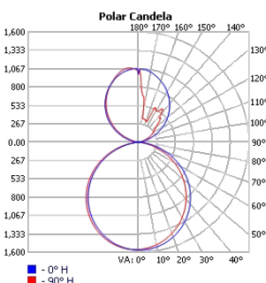
TECHOLED-BX-2-DI-6-HI-30
