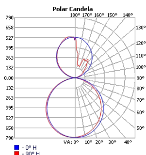
TECHOLED-BX-2-DI-6-LO-30
