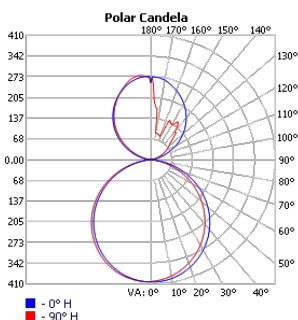
TECHOLED-BX-2-DI-2-ME-30
