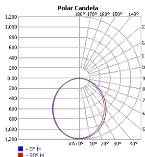
TECHOLED-BX-2-D-4-ME-30
